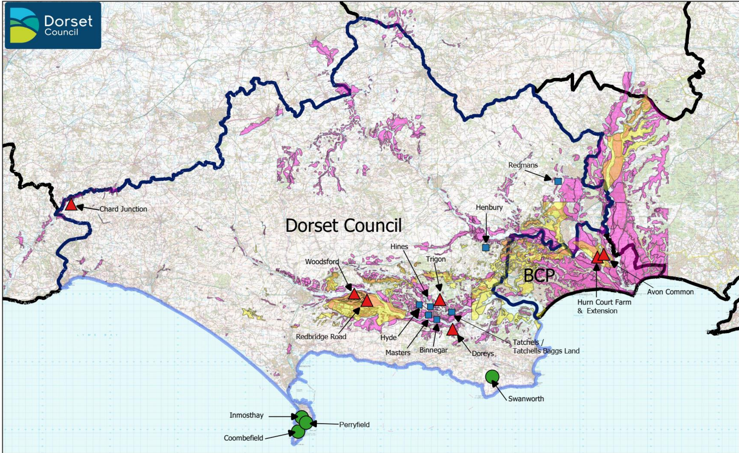
Figure 1A – The Sand and Gravel Resource, with permitted aggregate quarries in 2022
