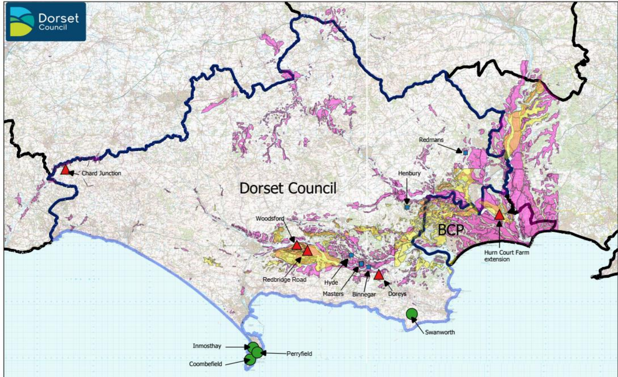
Figure 1 – The Sand and Gravel Resource, with aggregate quarries operational in 2022
