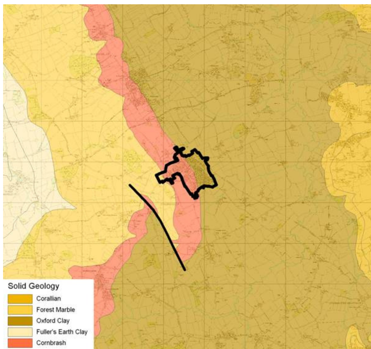
Figure 4: Geology of the Stalbridge Area.
